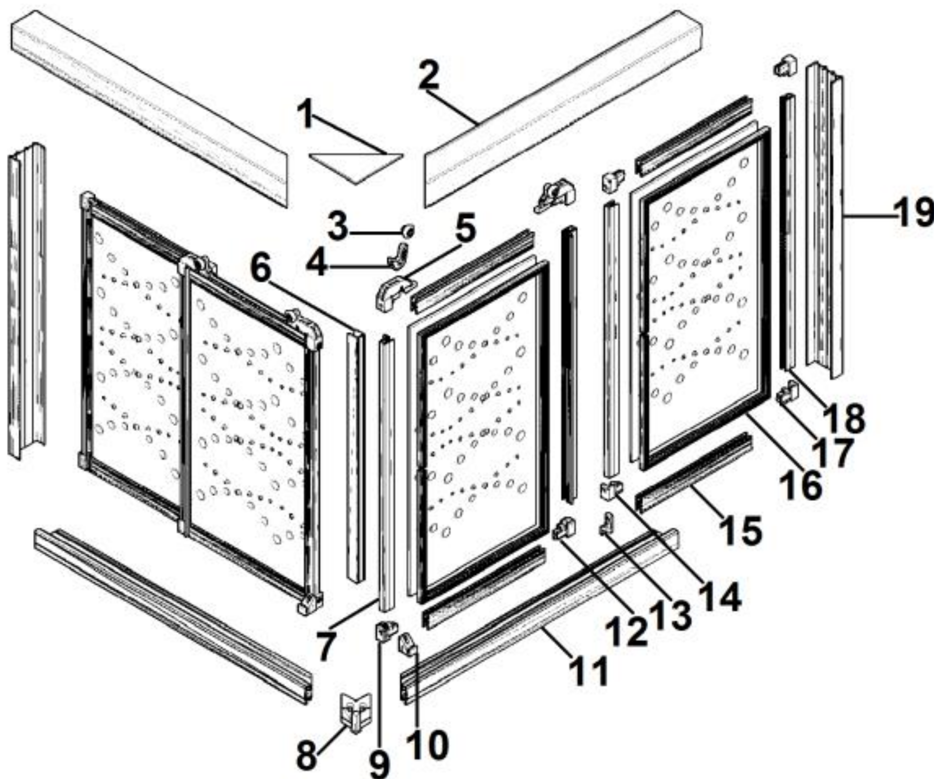
SHOWER SCREEN - CORNER ENTRY
