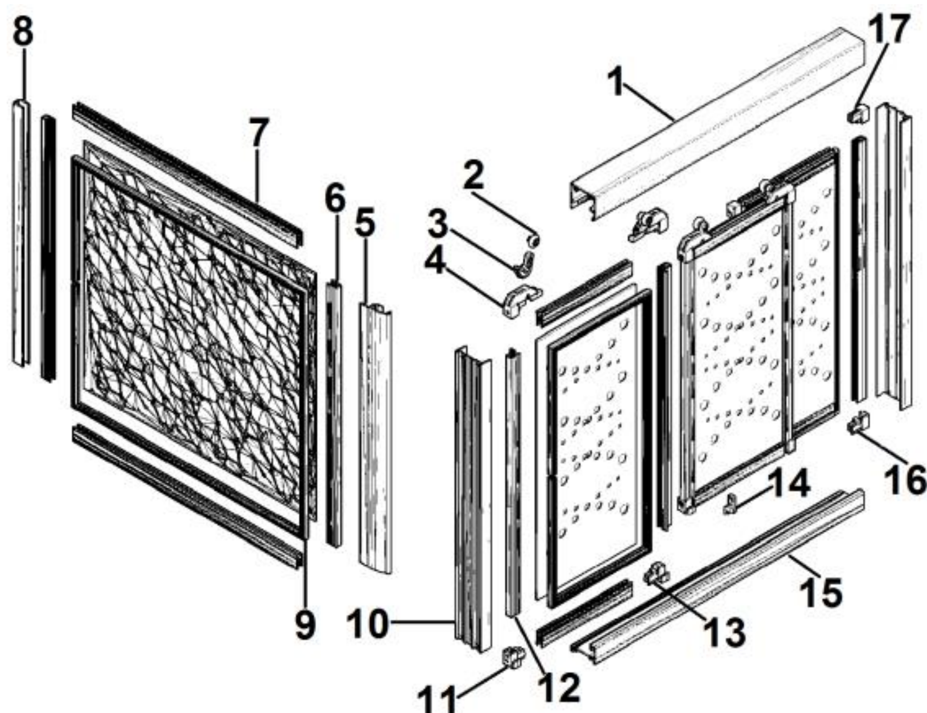
SHOWER SCREEN CORNER SCREEN
